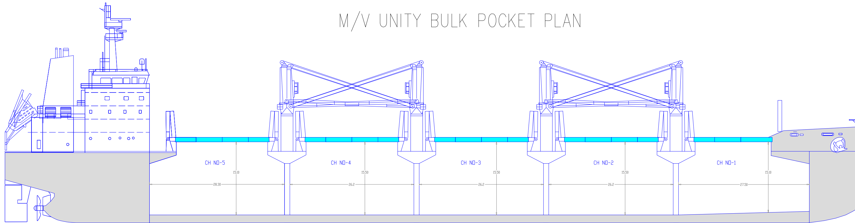
PROFILE VIEW
