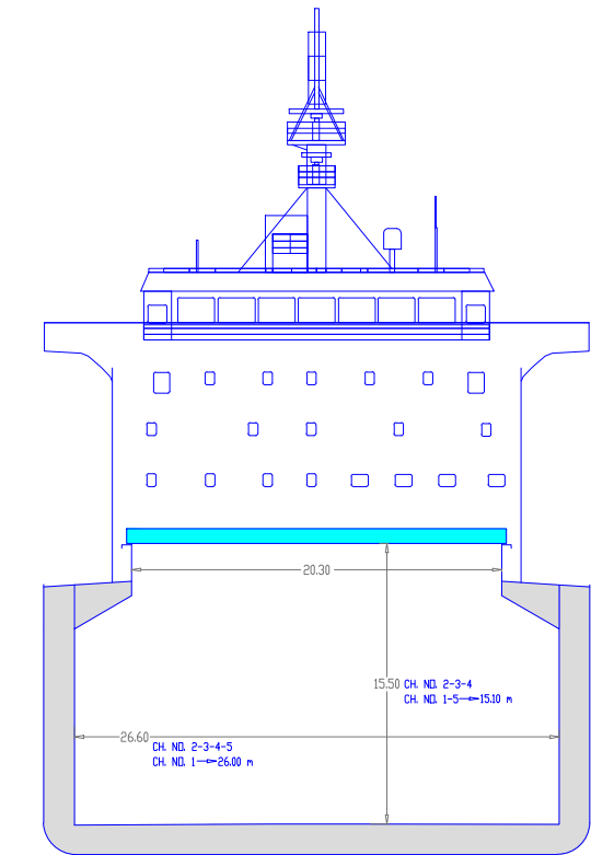
TRANSVERSE SECTION
